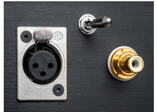
The power amplifier offers an unbalanced input as a standard feature, which is realized with first-class RCA jacks from WBT. If desired, a balanced XLR input can also be installed. A toggle switch with fuse is then used for switching: Only when you first pull the head out a little can the switch be flipped.
