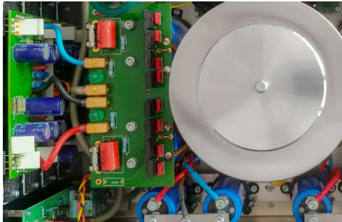
A look under the hood: Here we see the upper of the two super-imposed Mu-metal transformers. Extra-potent versions come into play for the Anniversary Edition: Each of these transformers is capable of delivering 800 volt-amps – adding up to a whopping 1,600 volt-amps. Beneath them, you can see the smaller electrolytic capacitors, which serve as a buffer for the large electrolytic capacitors of the power supply. Their connection via metal rails ensures better energy dissipation. Otherwise, Symphonic Line uses extremely high-quality conductor material for the connection, which is also used in the maker's signal cables.
